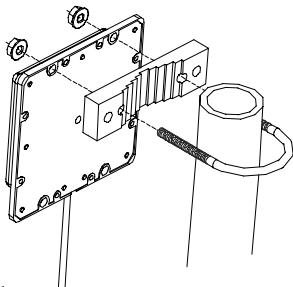
HGX-PMT07 - Stationary Mounting Kit for mast mounting
